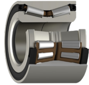
Hub bearing unit (HBU1T) Type 5
