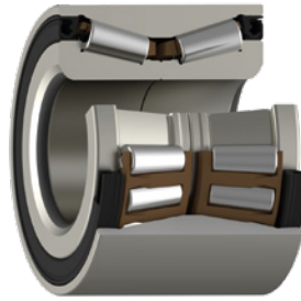
Hub bearing unit (HBU1T) Type 5
